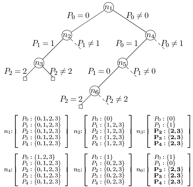
Figure 1: Pigeon holes: partial search tree
