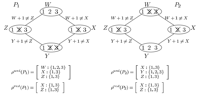
Figure 3: Network reduction by \rho^{uni} and \rho^{red}
